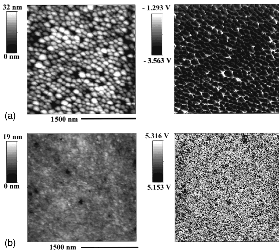
Figure 14. AFM (left) and KFM (right) images of the larger (about 141 nm, top) and smaller (about 36 nm, bottom) Stober silica particles.
